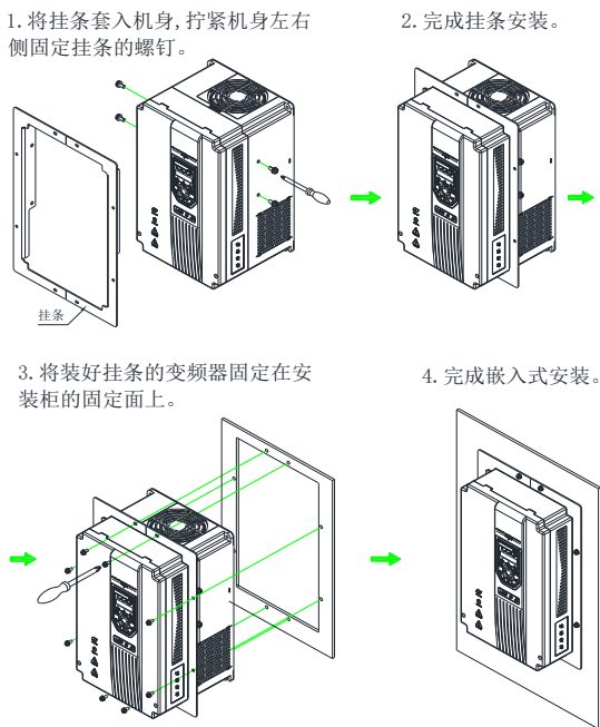
图 3-8 Hope500PM11T4~Hope500PM37T4 机型嵌入式安装
