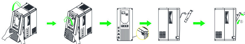
图 3-10 Hope500PM0.75T4~Hope500PM7.5T4 机型盖板拆卸与安装步骤
