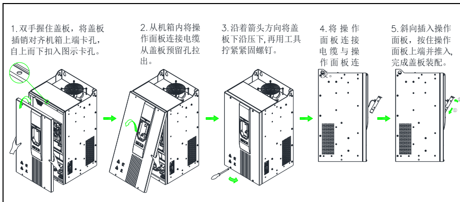
图 3-12 Hope500PM45T4~Hope500PM160T4 机型盖板拆卸与安装步骤
