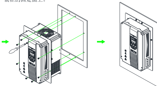
图 3-8 Hope500PM11T4~Hope500PM37T4 机型嵌入式安装
