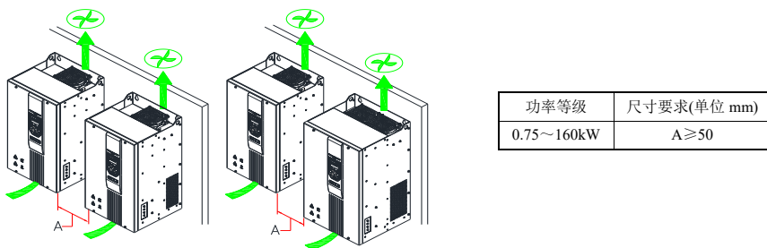
图 3-3 Hope500PM0.75T4~Hope500PM160T4 多台机器并排安装
