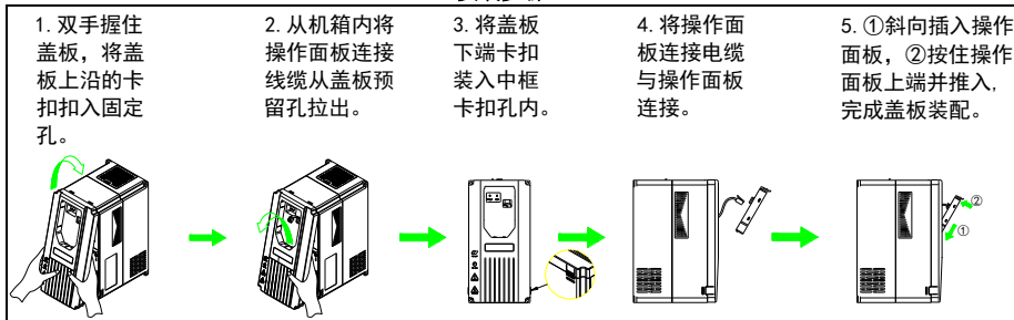
图 3-10 Hope530G0.75T4~Hope530G7.5T4 机型盖板拆卸与安装步骤
