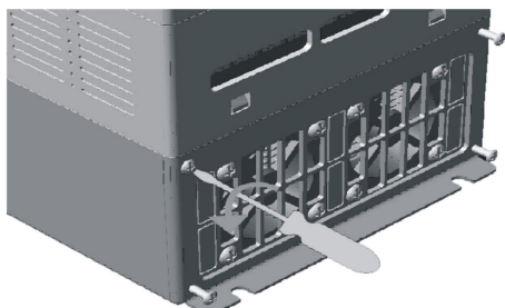
旋松端盖板螺钉
